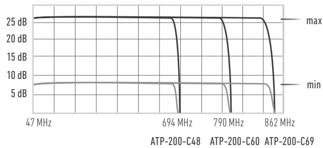
Graphs of gain control
